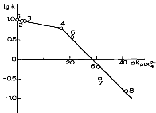
Fig. 4. Rate of cyclohexane H-D exchange ( \text{l mol}^{-1} \text{sec}^{-1} , in systems \text{PtCl}_2 + 2\text{X}^- ) vs. stability constants of \text{PtX}_4^{2-} ; \text{X} = \text{H}_2\text{O} (1), \text{F}^- (2), \frac{1}{2}\text{SO}_4^{2-} (3), \text{Cl}^- (4), \text{Br}^- (5), \text{I}^- (6), \text{NO}_2^- (7), \text{CN}^- (8).
