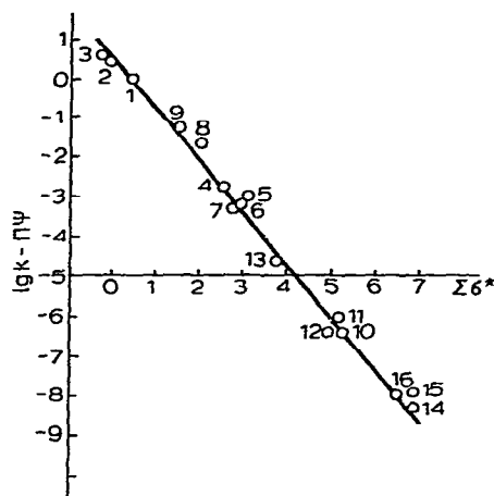
Fig. 3. Rate of H-D exchange (% h -1 ) vs. Taft polar constants of H-CXY 2 ; X = H, CH 3 , C 2 H 5 , CF 3 , OH, COOH, Y; Y = H, F, Cl, Br. ( n = 0:1 = methane, 2 = ethane, 3 = propane, 4 = 1,1,1-trifluoroethane; n = 1:5 = fluoromethane, 6 = chloromethane, 7 = bromomethane, 8 = acetic acid, 9 = methanol; n = 2:10 = difluoromethane, 11 = dichloromethane, 12 = fluorochloromethane, 13 = 1,1-difluoroethane; n = 3:14 = trifluoromethane, 15 = trichloromethane, 16 = tribromomethane).
