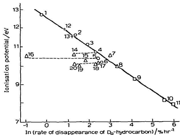
Fig. 2. Rate of H—D exchange versus ionization potential of alkanes and aromatic compounds (1 = methane, 2 = ethane, 3 = propane, 4 = n-butane, 5 = n-pentane, 6 = n-hexane, 7 = cyclopentane, 8 = cyclohexane, 9 = benzene, 10 = naphthalene, 11 = phenanthrene, 12 = 2,2-dimethylbutane, 13 = 1,1-dimethylpropylbenzene, 14 = 2-methylpropane, 15 = 2-methylbutane, 16 = 2,2-dimethylpropane, 17 = 2-methylpentane, 18 = 3-methylpentane, 19 = 2,3-dimethylbutane, 20 = 2,2-dimethylbutane).
