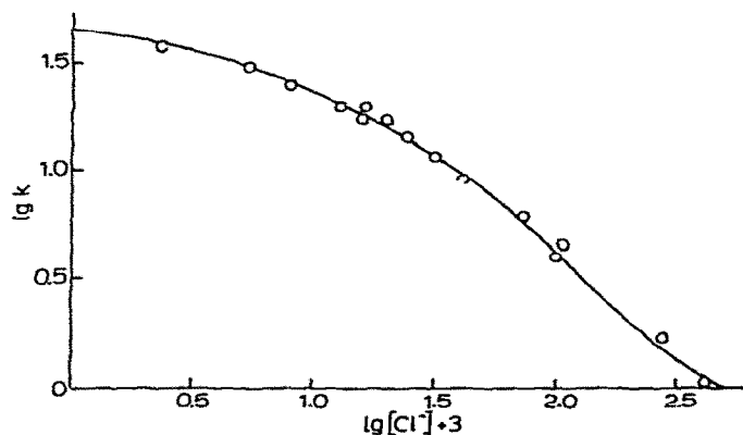
Fig. 5. Rate of cyclohexane H-D exchange ( 1 \text{ mol}^{-1} \text{ sec}^{-1} ) versus chloride ion concentration ( \text{mol l}^{-1} ) (points = experimental values, solid line = calculated at k_1:k_2:k_3 = 100:14:0.6 , K_1 = 3 \cdot 10^{-2} , K_2 = 5 \cdot 10^{-2} \text{ mol l}^{-1} ).
